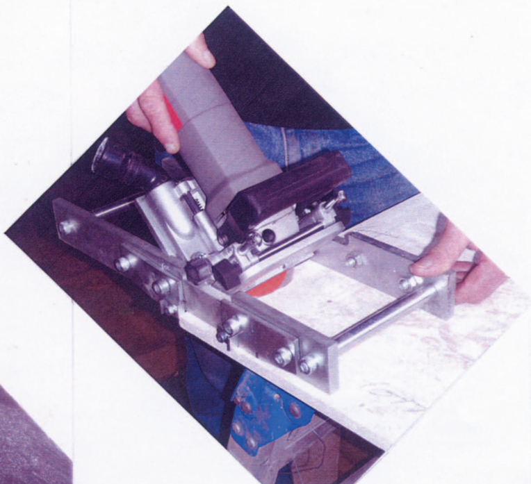
SUPPORTCLIP-CUTTER INSERTING BOTTOM CUT IN PANEL
